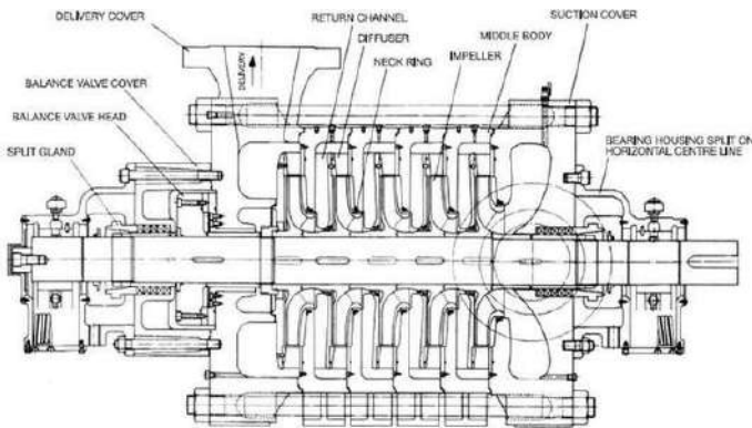
SECTION THROUGH TYPICAL PL/PJ PUMP
