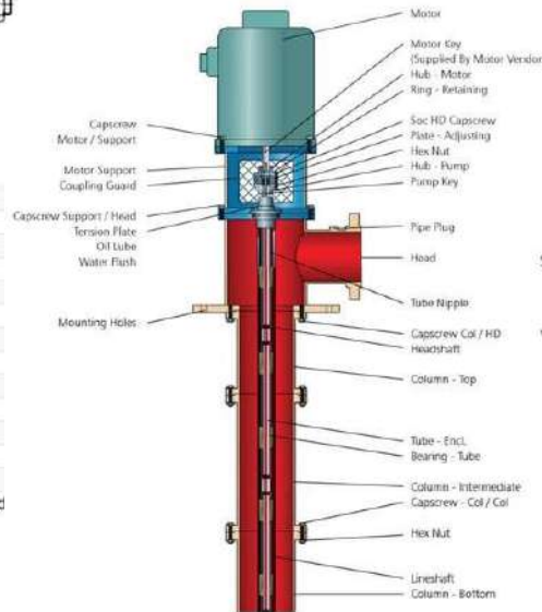
SECTION THROUGH TYPICAL PL/PJ PUMP
